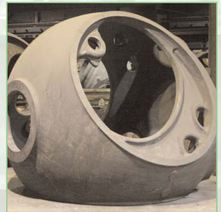
Wind Turbine Hub (30,000 lbs.)
